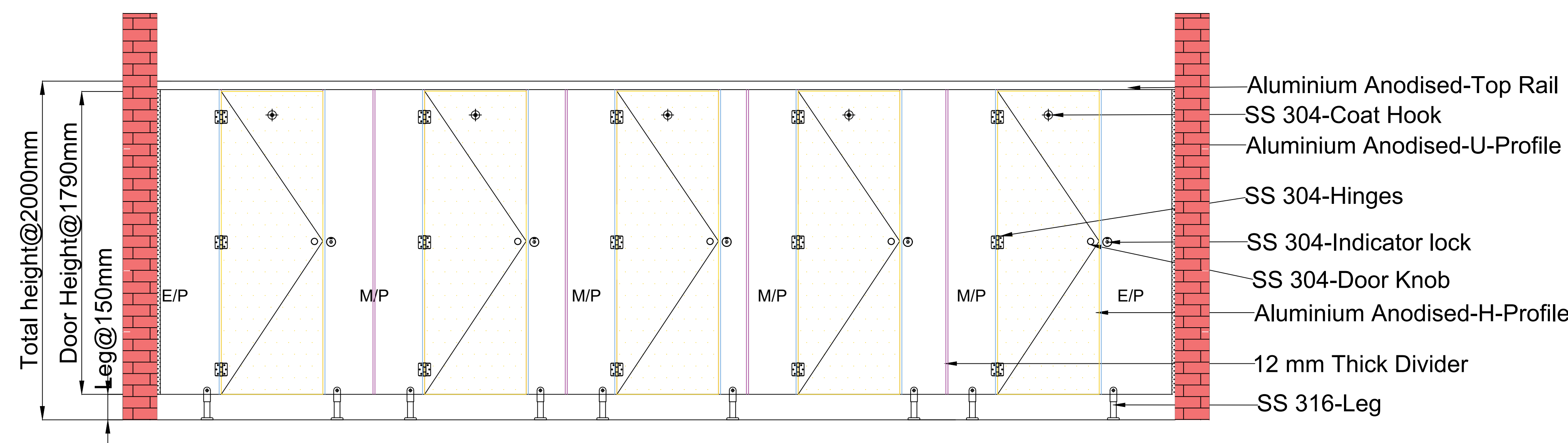
ELEVATION-AA
