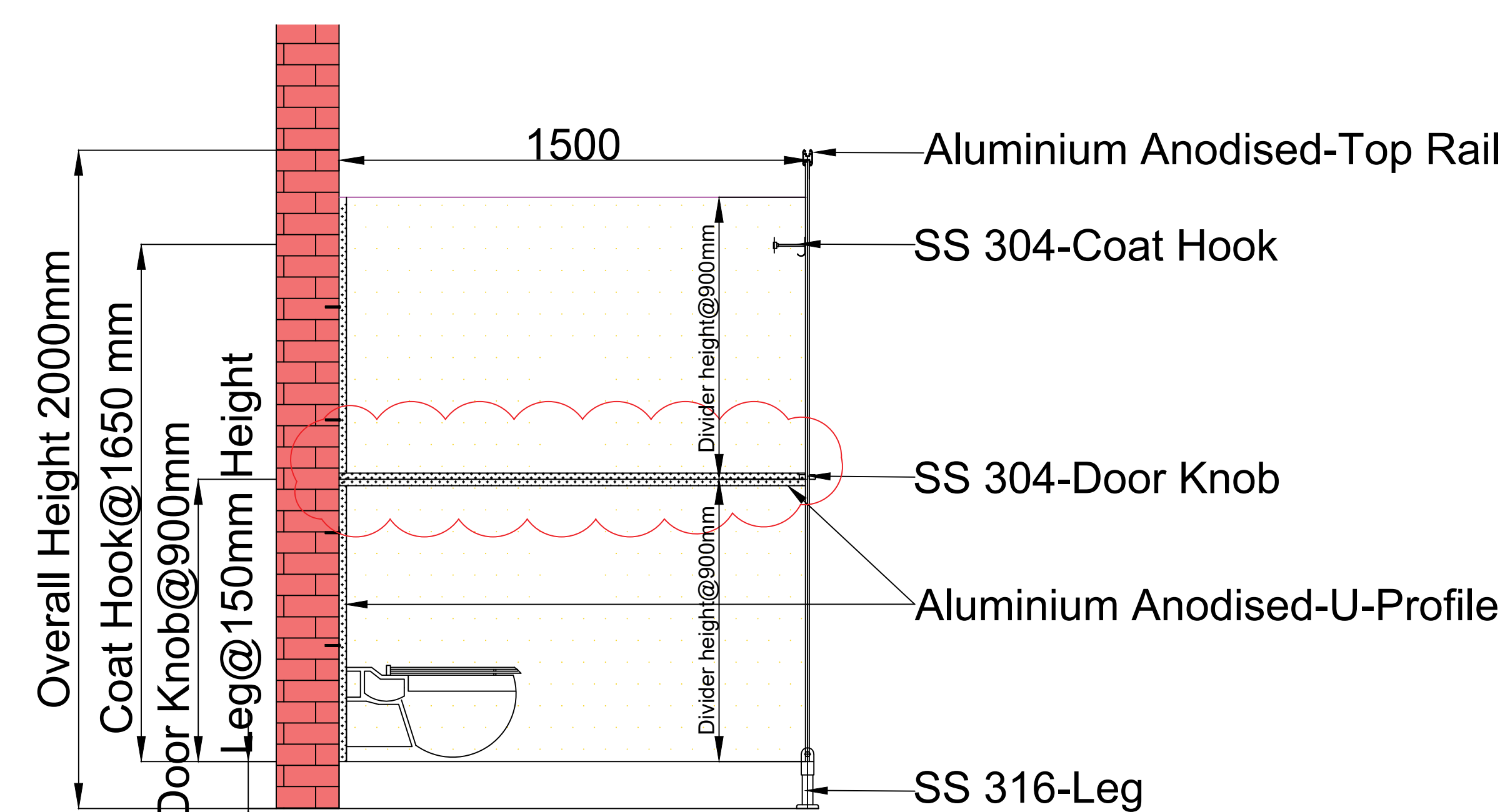
SECTION-BB
