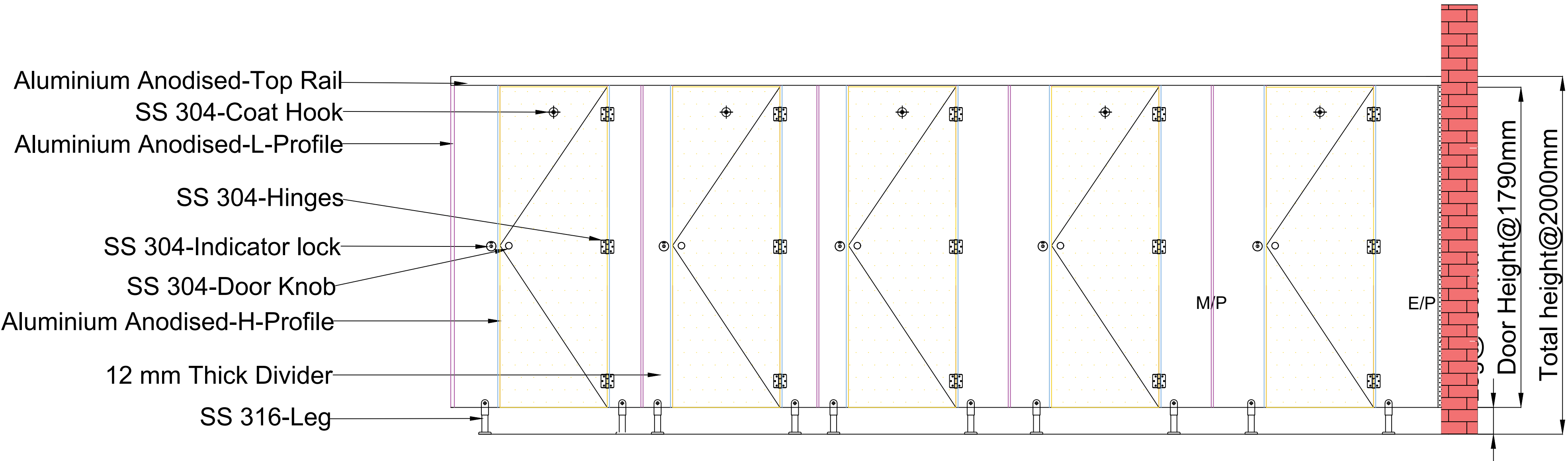
ELEVATION-AA
