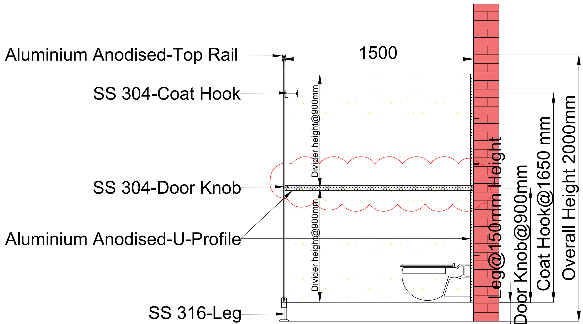
SECTION-BB
