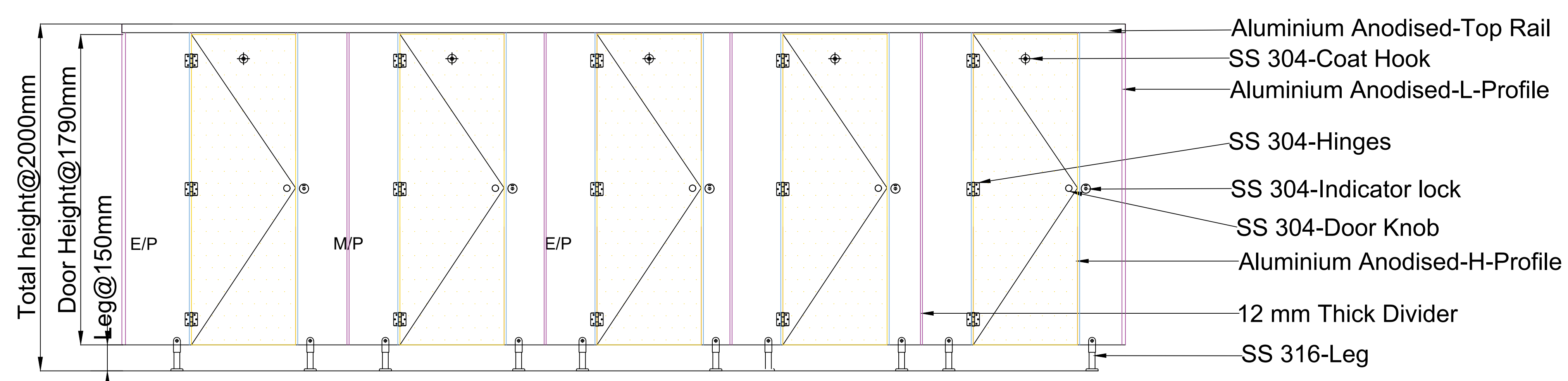
ELEVATION-AA
