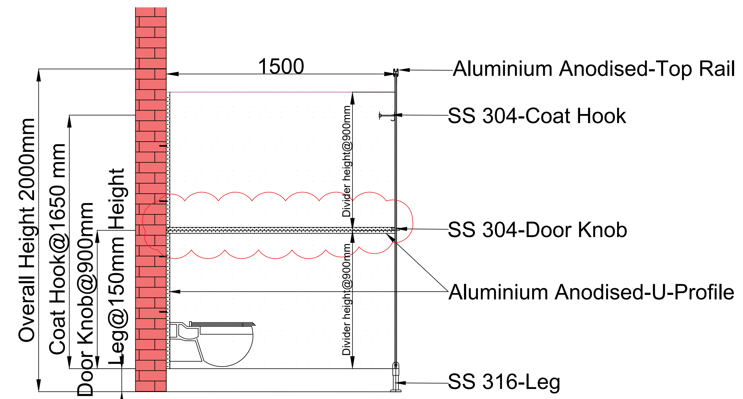
SECTION-BB
