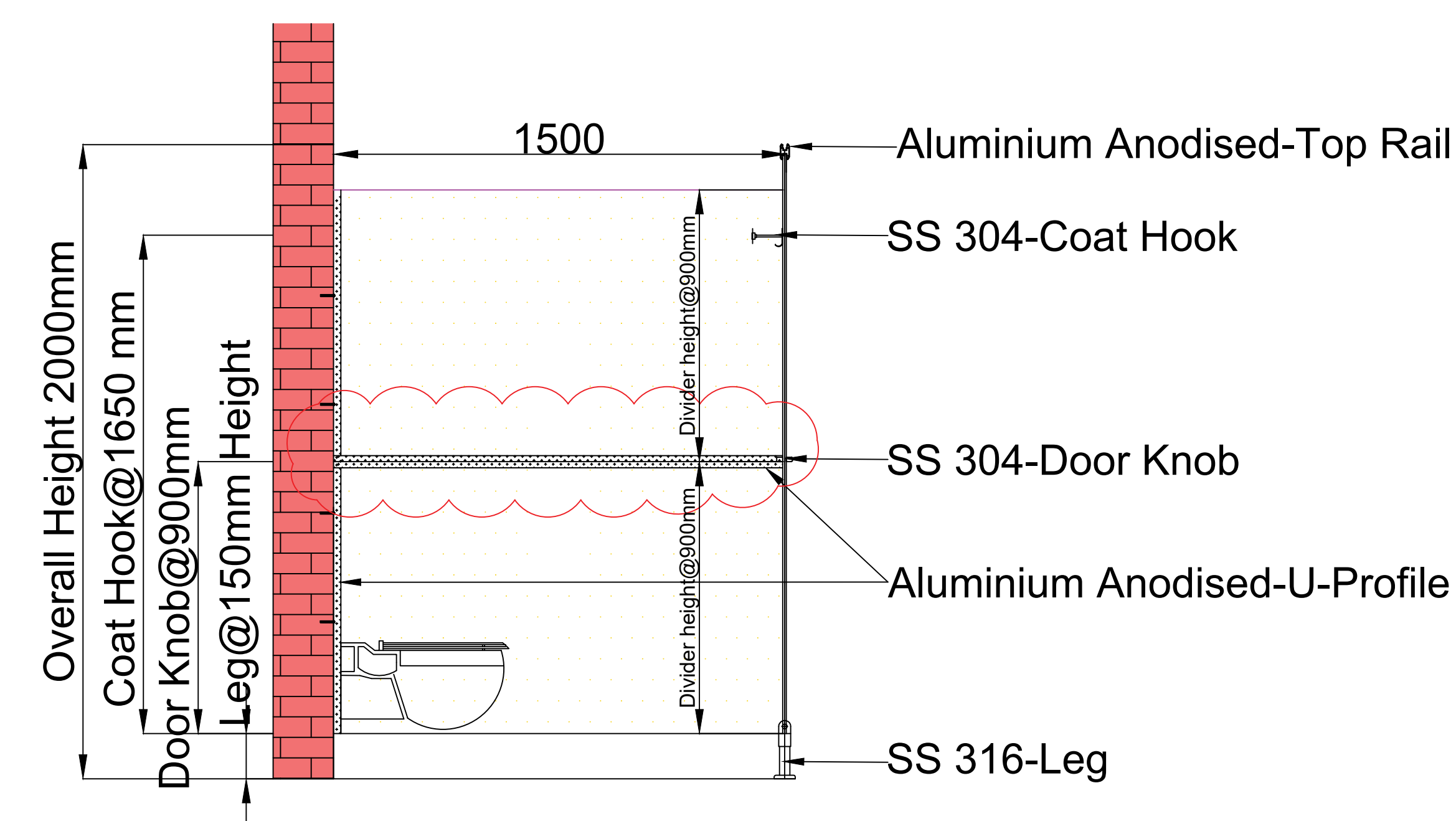
SECTION-BB
