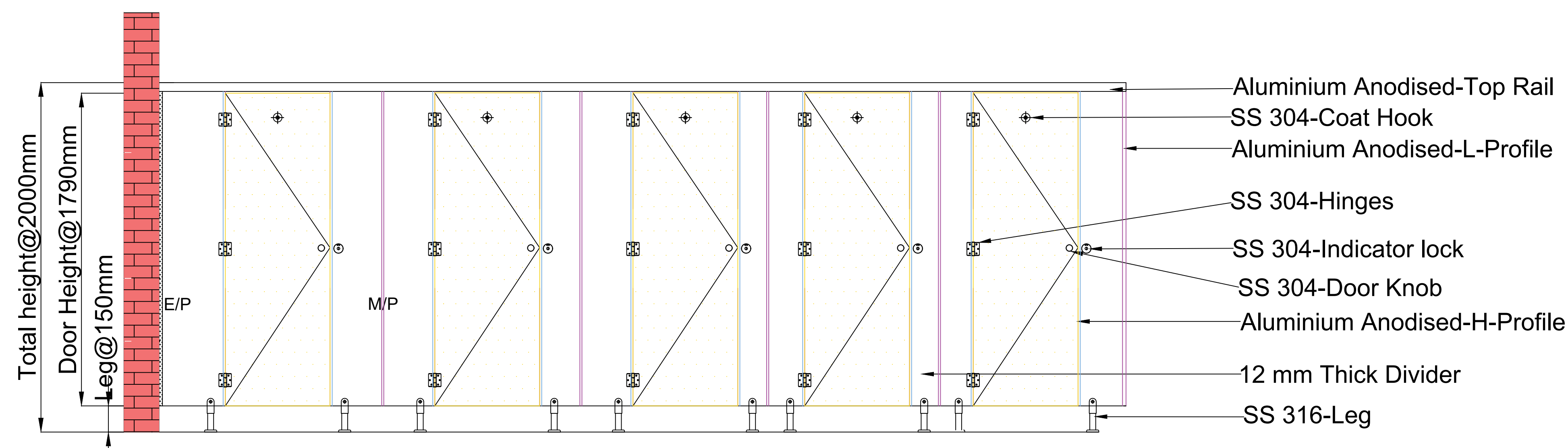
ELEVATION-AA
