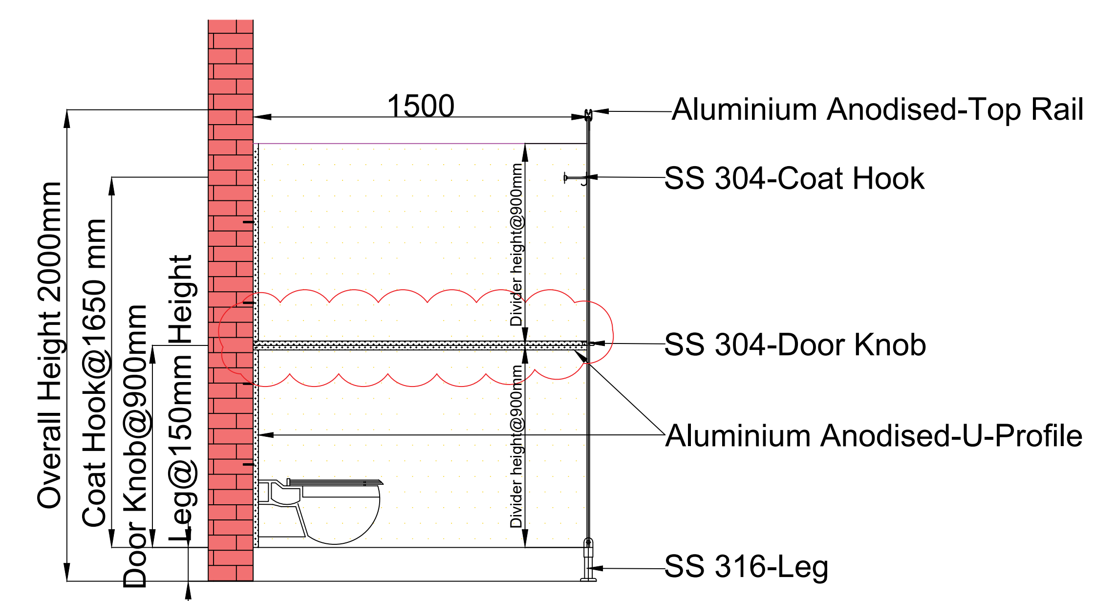
SECTION-BB
