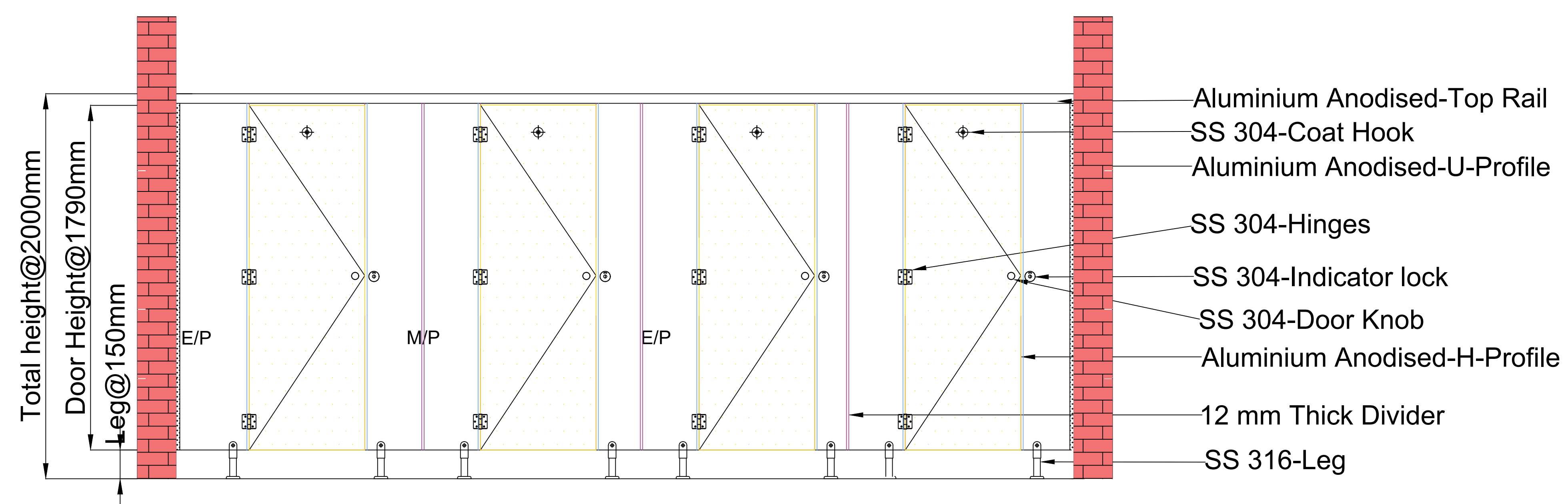
ELEVATION-AA
