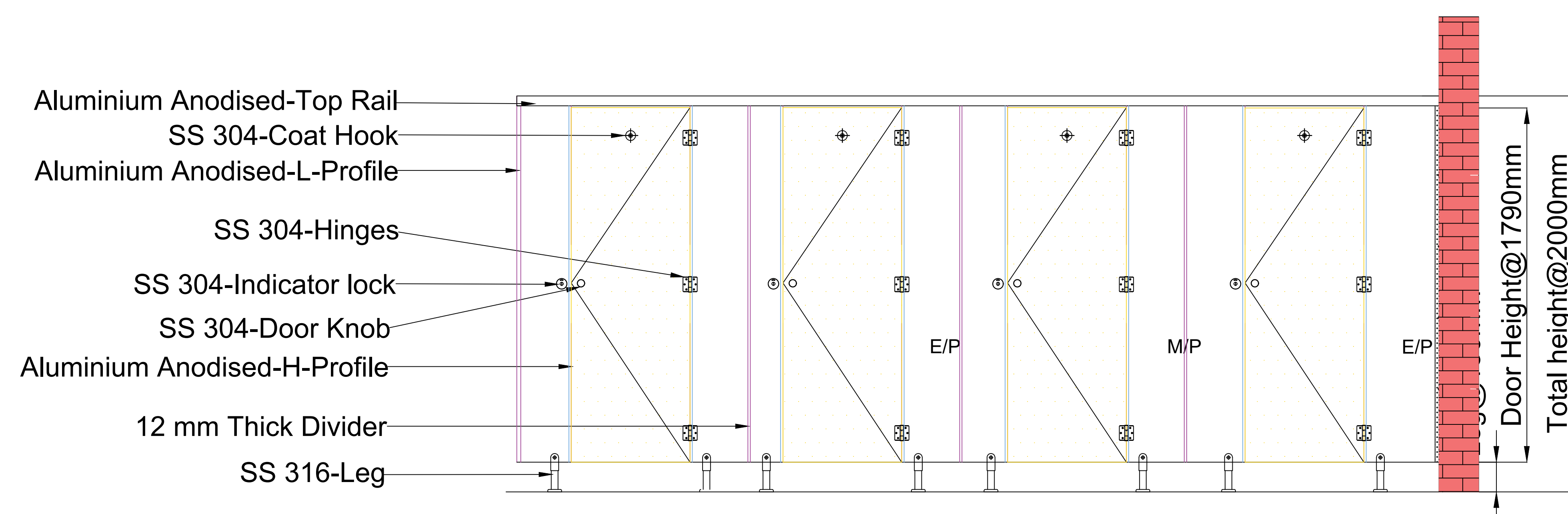
ELEVATION-AA
