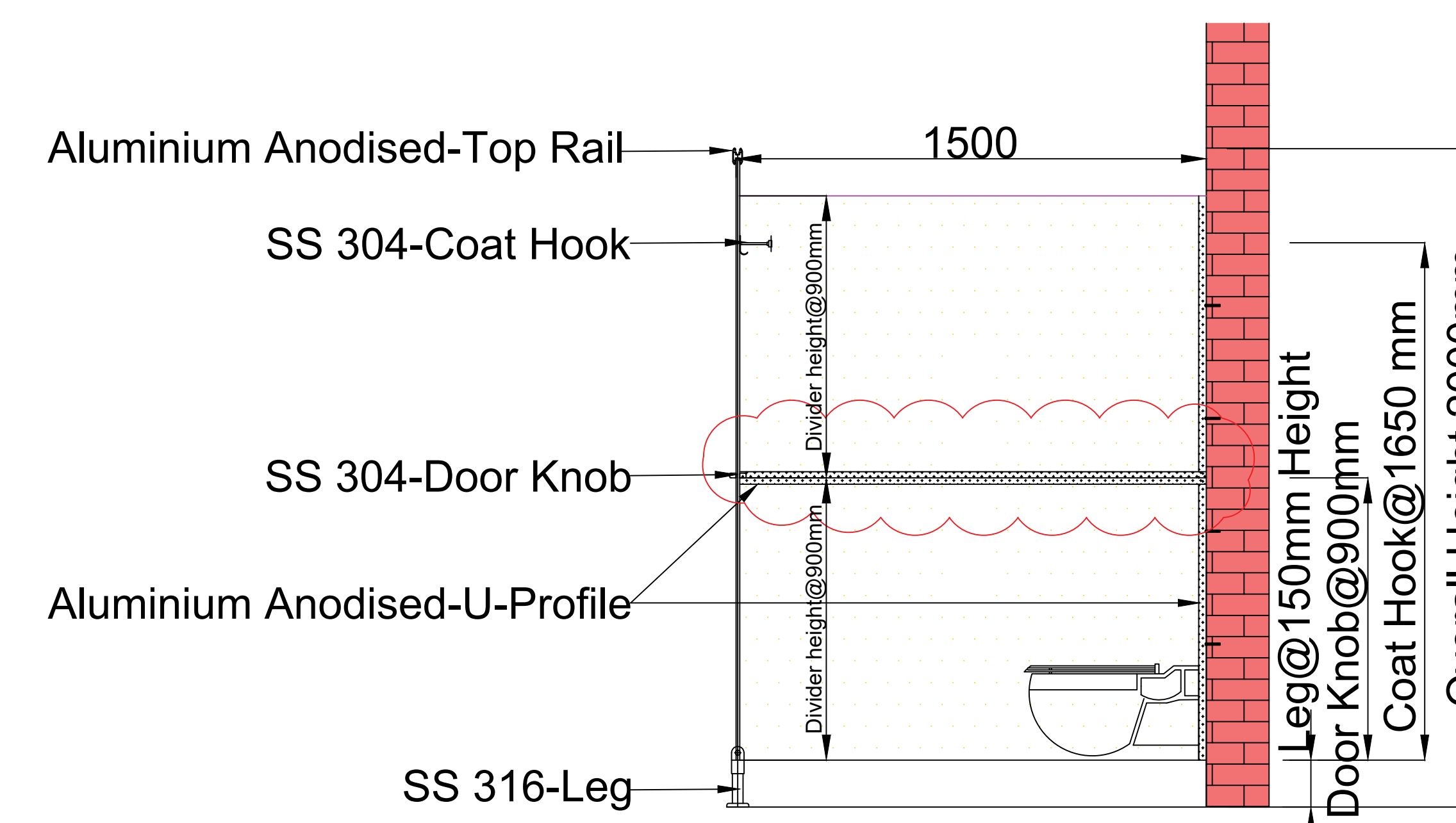
SECTION-BB
