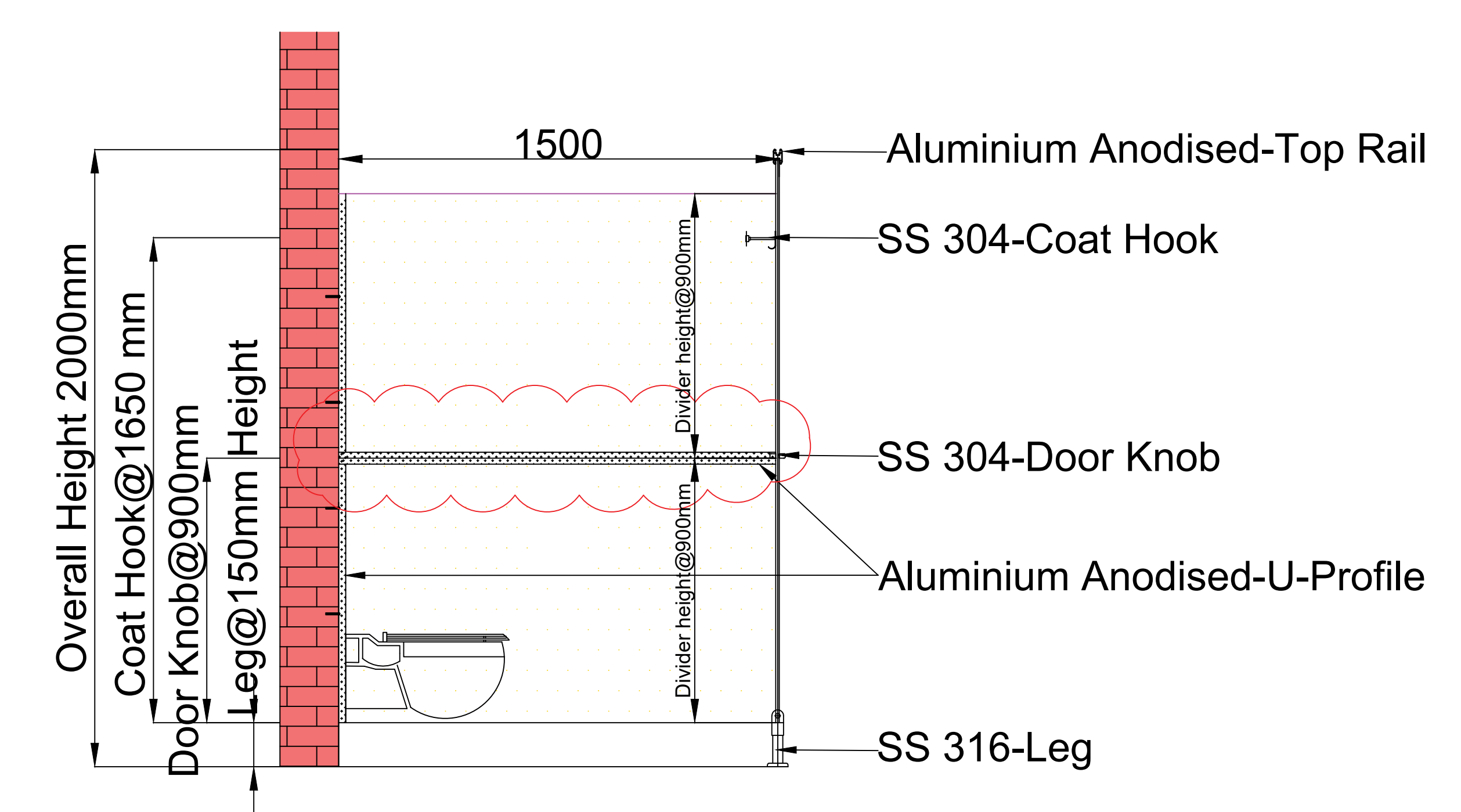
SECTION-BB
