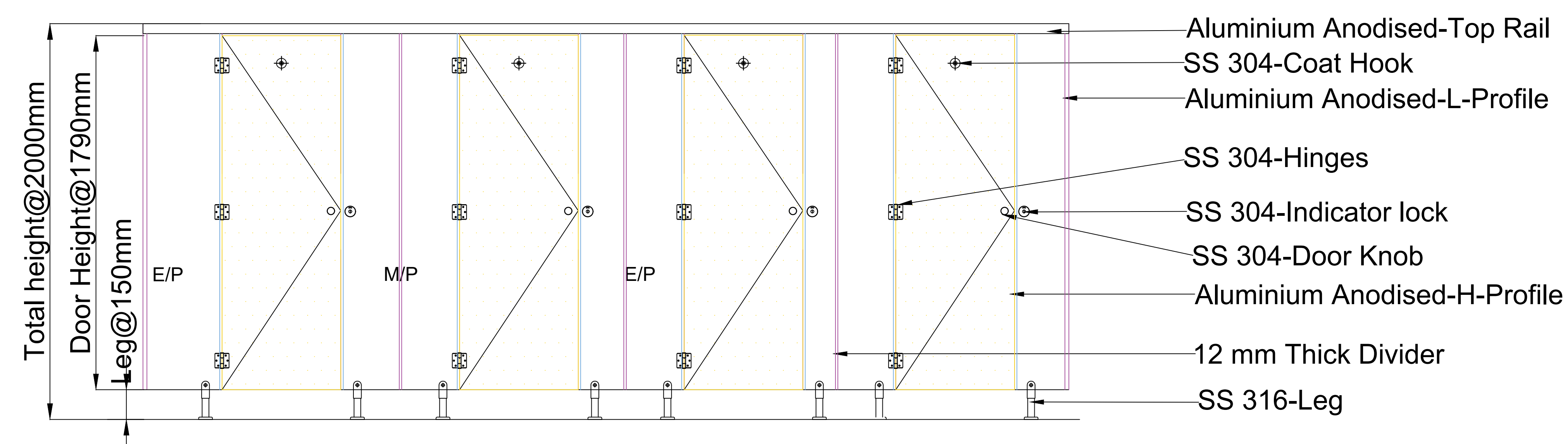
ELEVATION-AA
