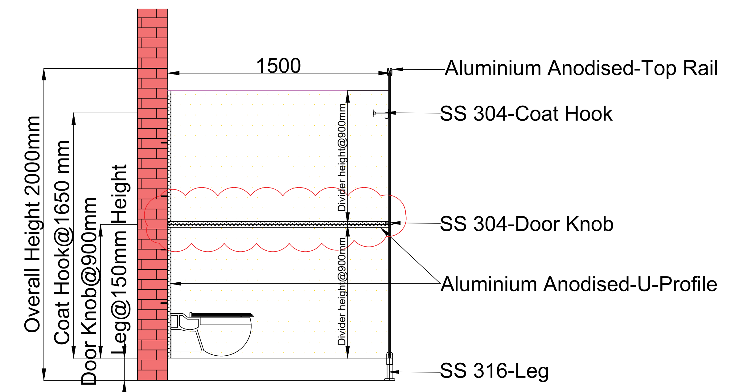
SECTION-BB
