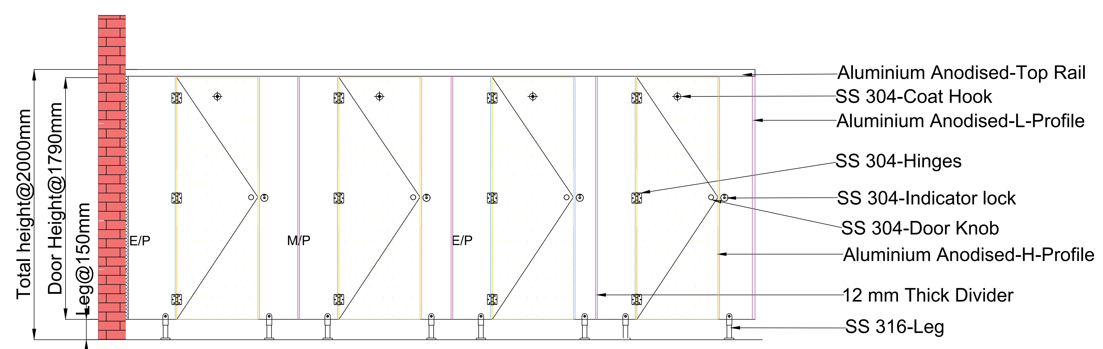
ELEVATION-AA
