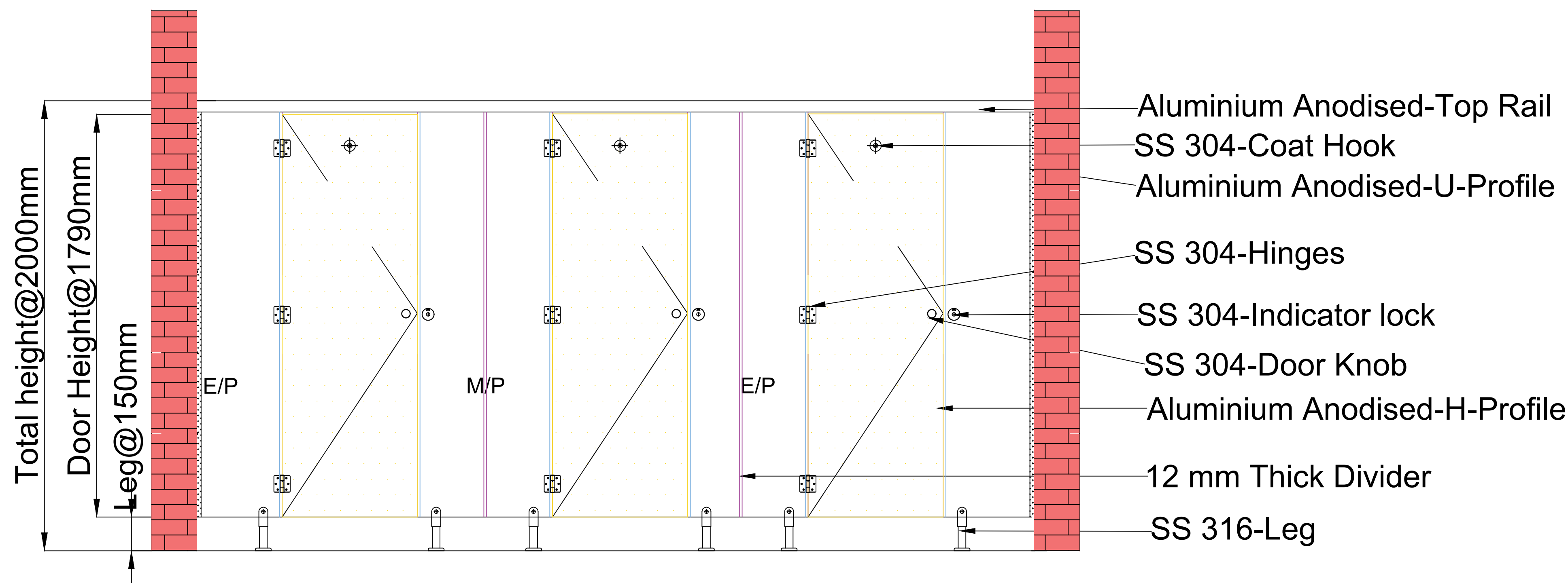
ELEVATION-AA
