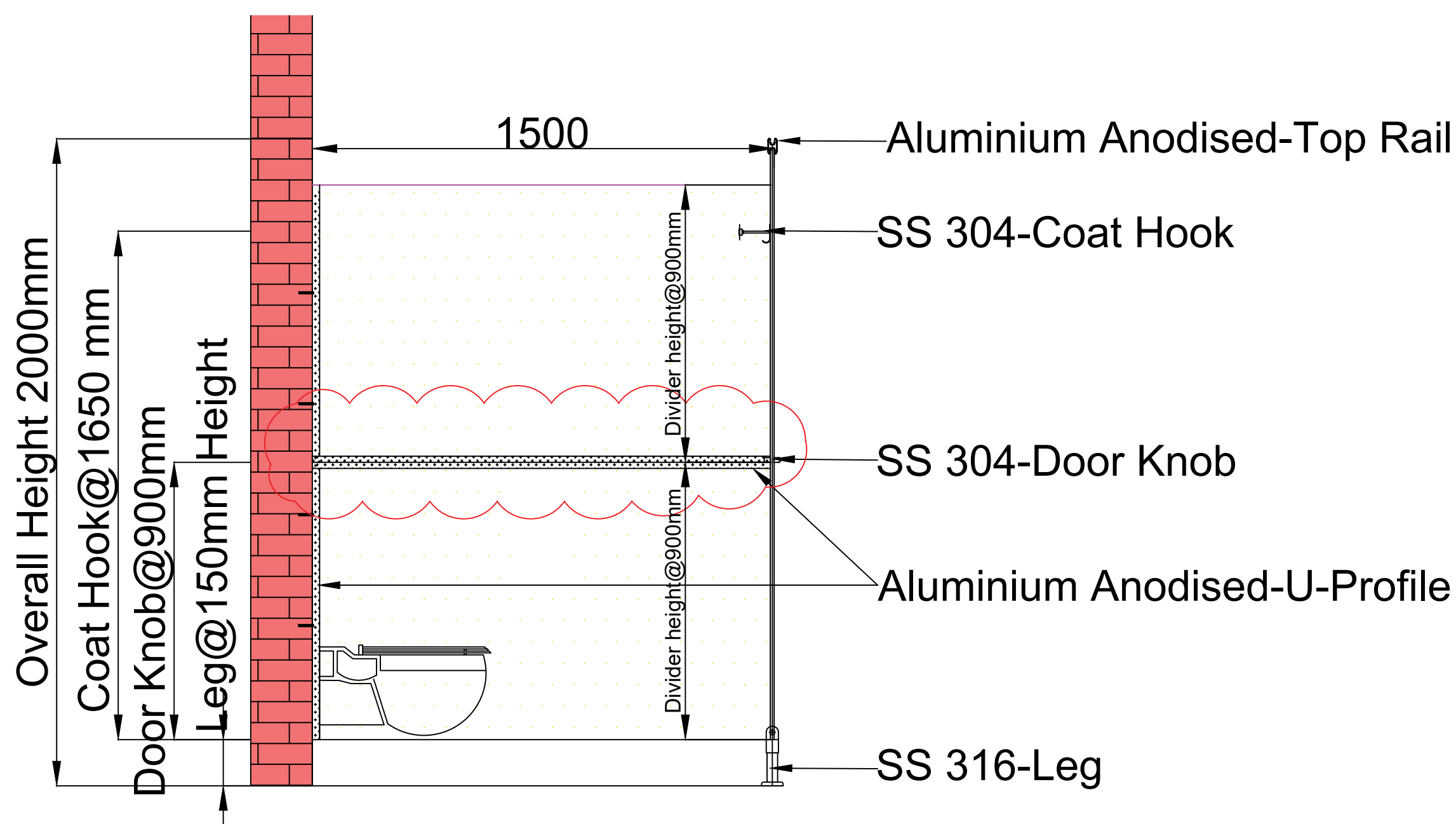
SECTION-BB
