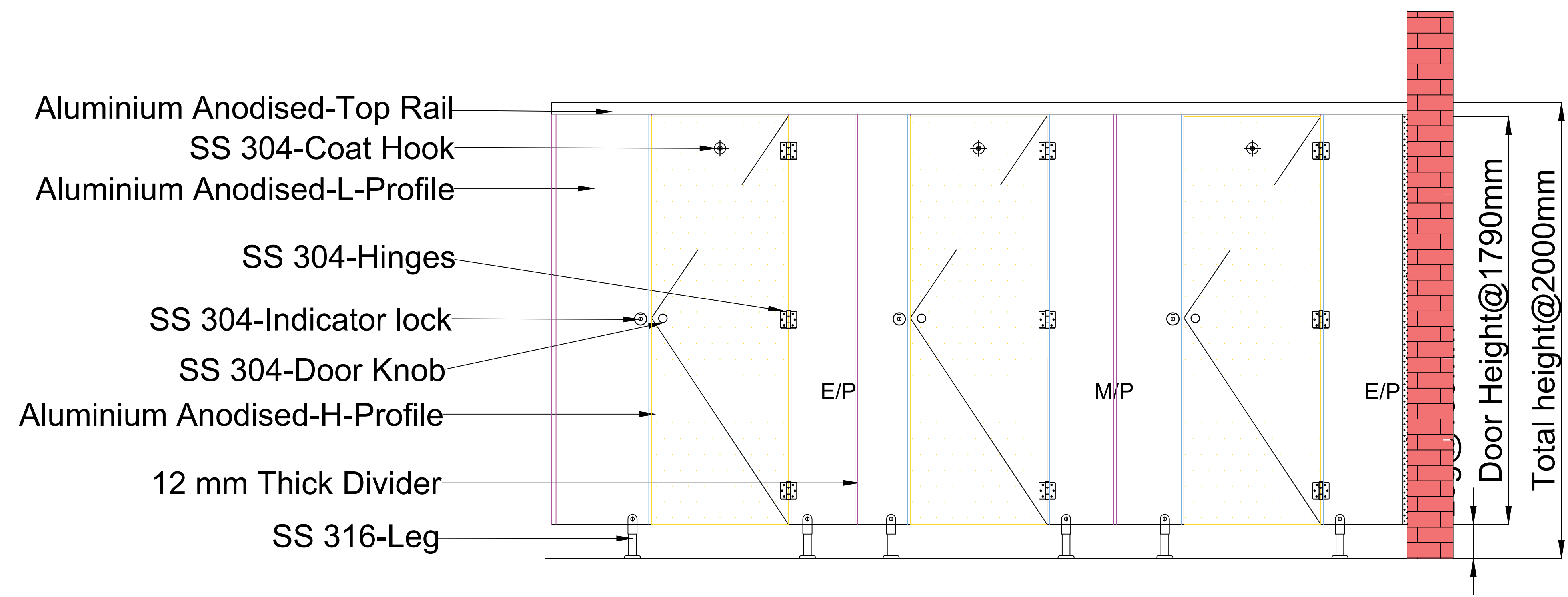
ELEVATION-AA
