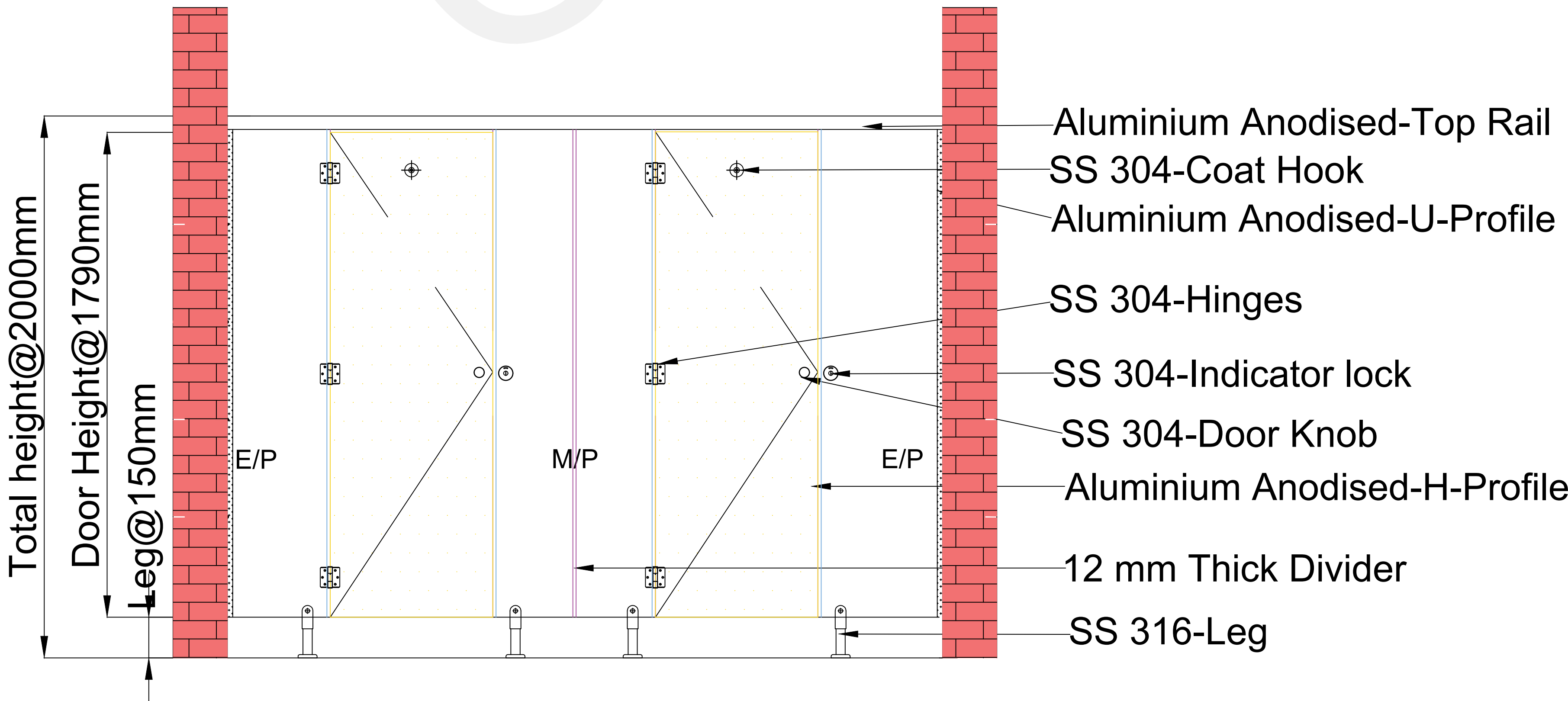
ELEVATION-AA
