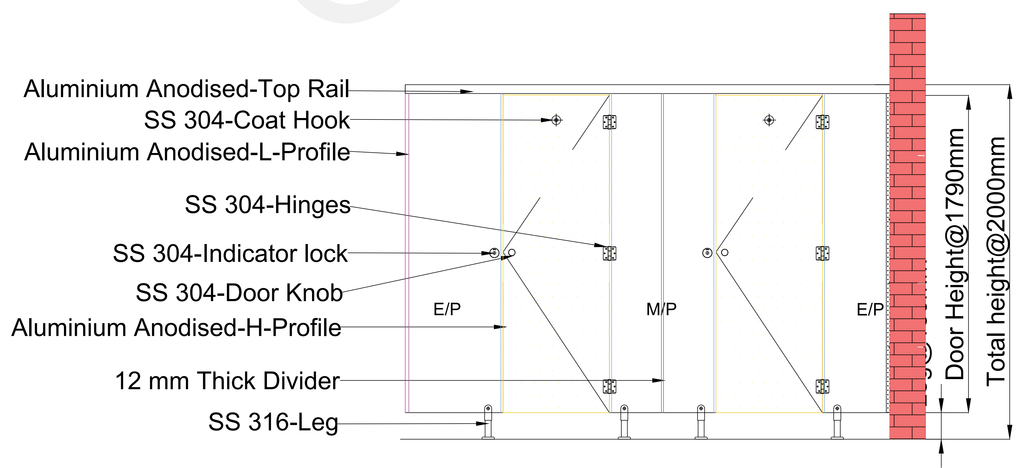
ELEVATION-AA
