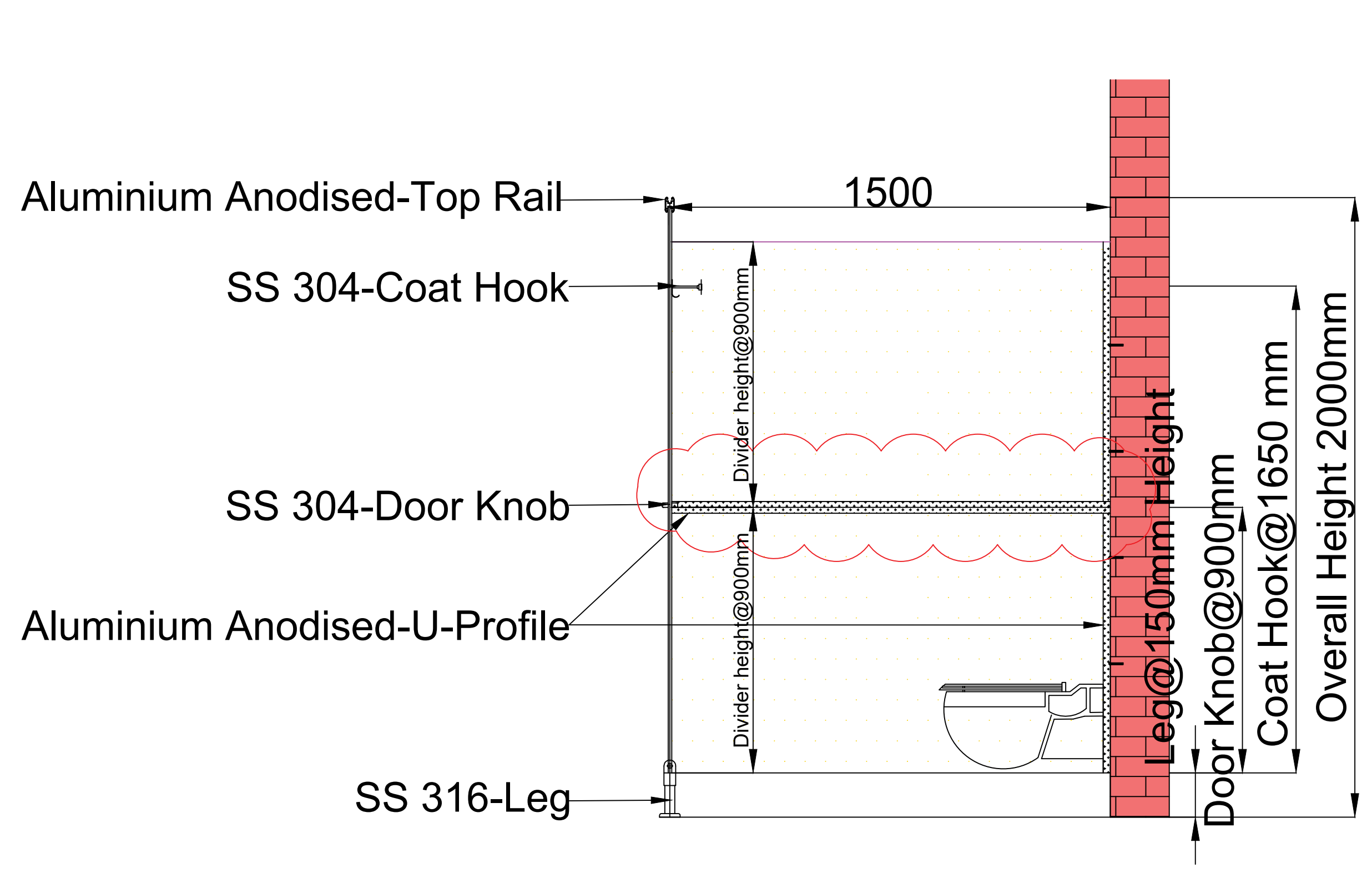
SECTION-BB
