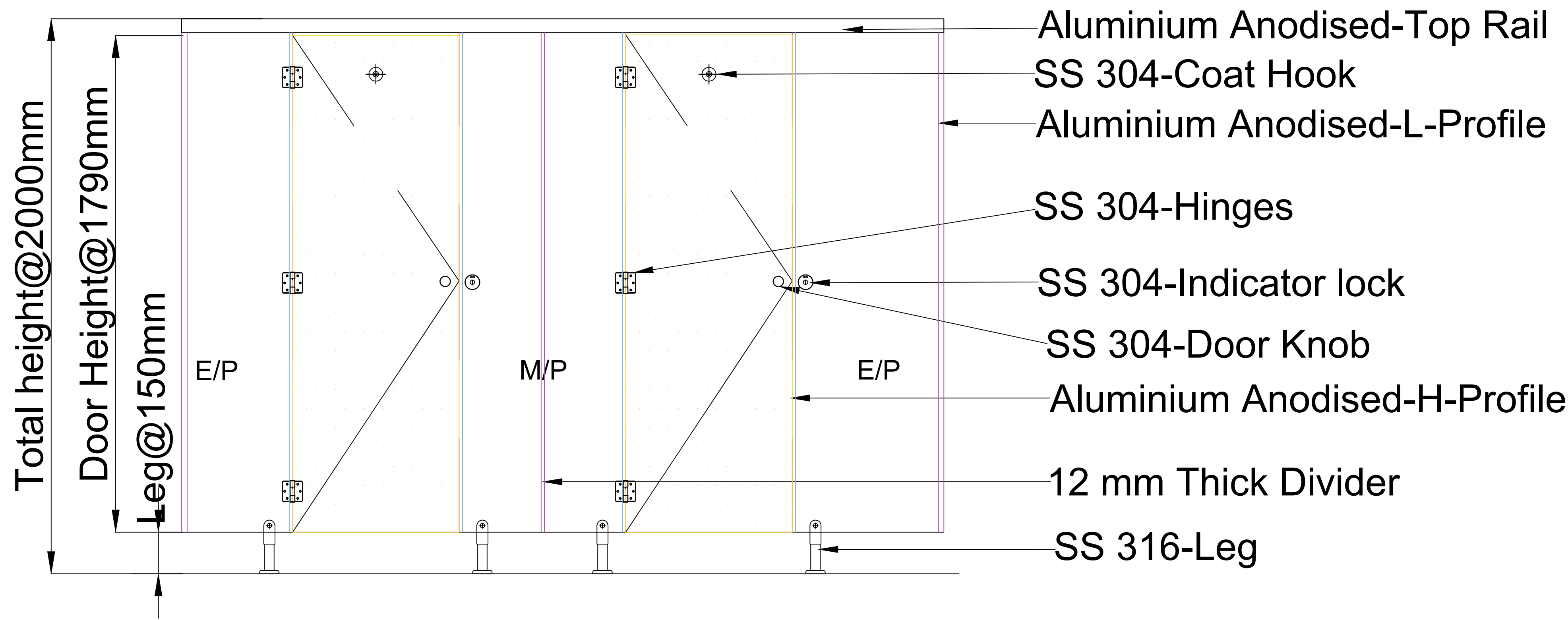
ELEVATION-AA
