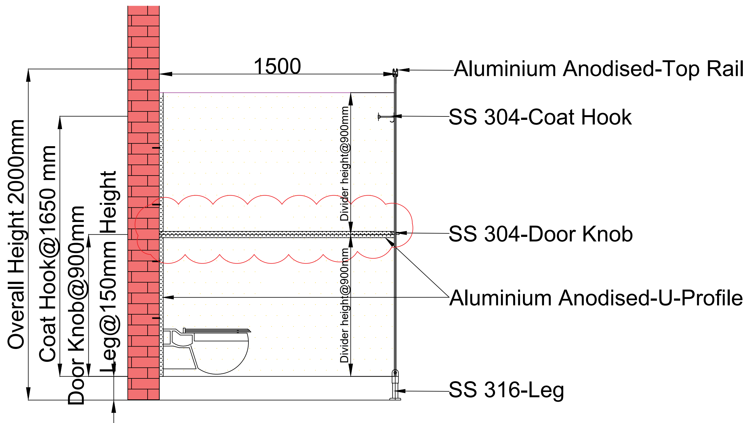
SECTION-BB
