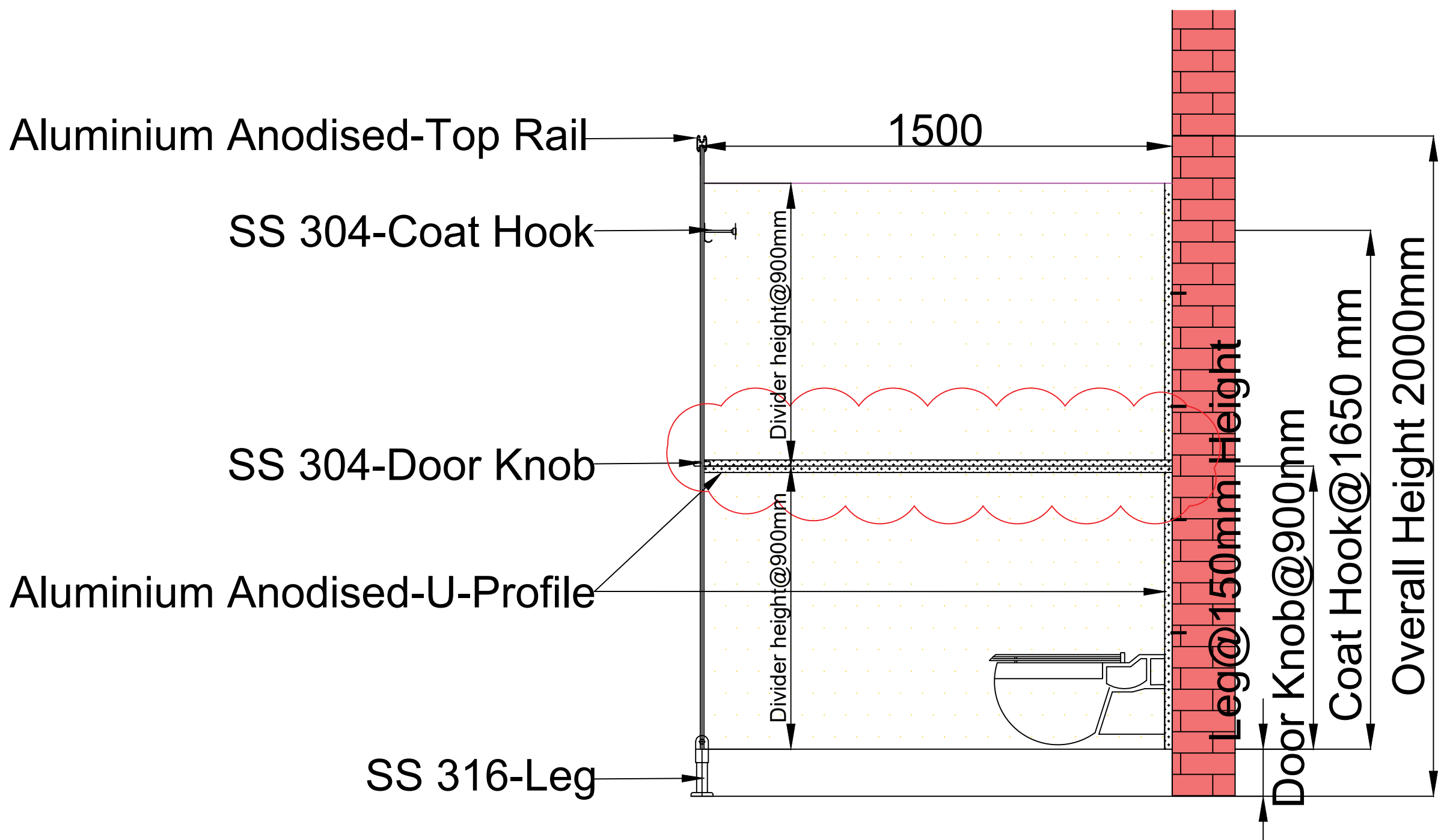
SECTION-BB
