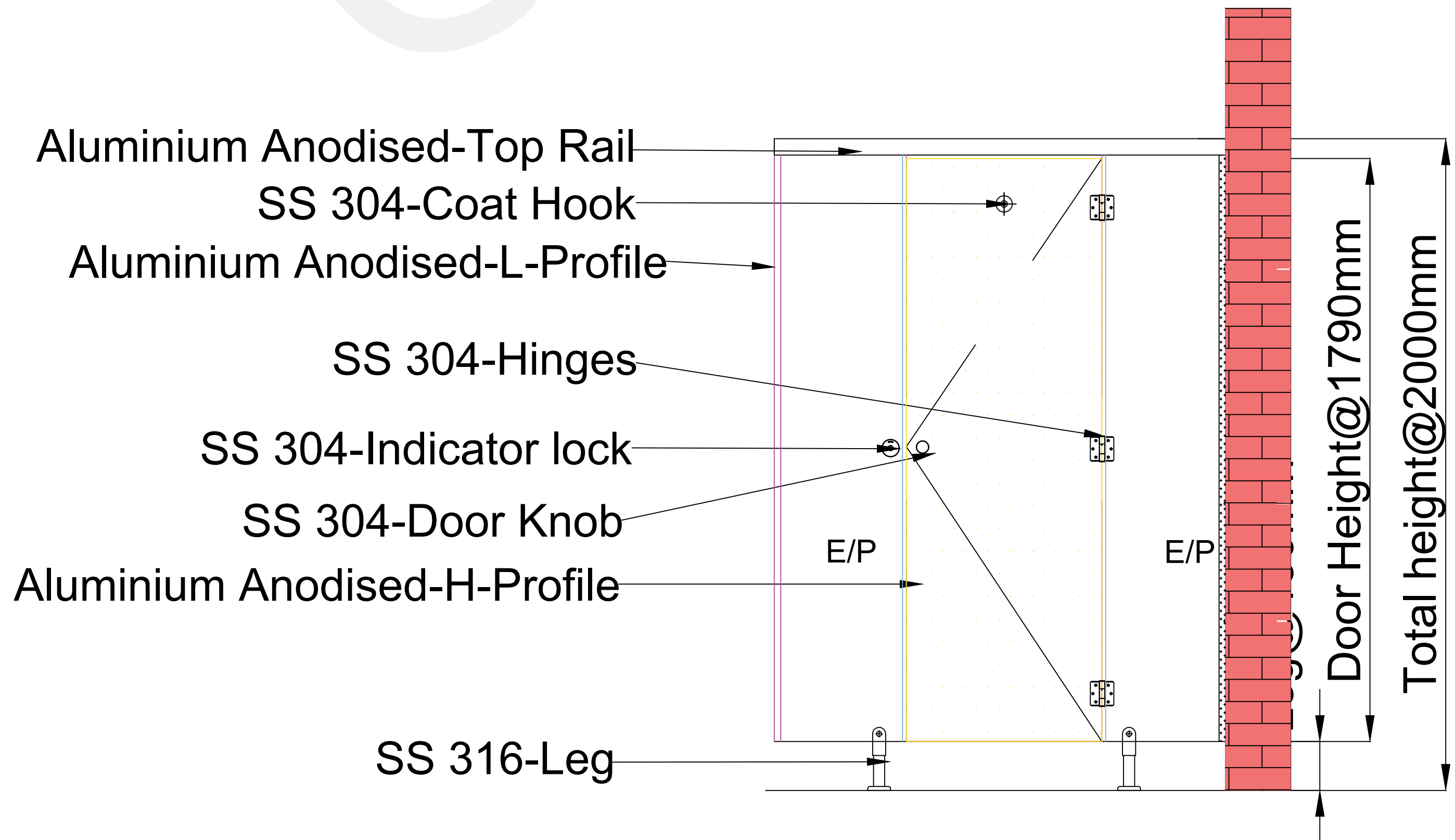
ELEVATION-AA
