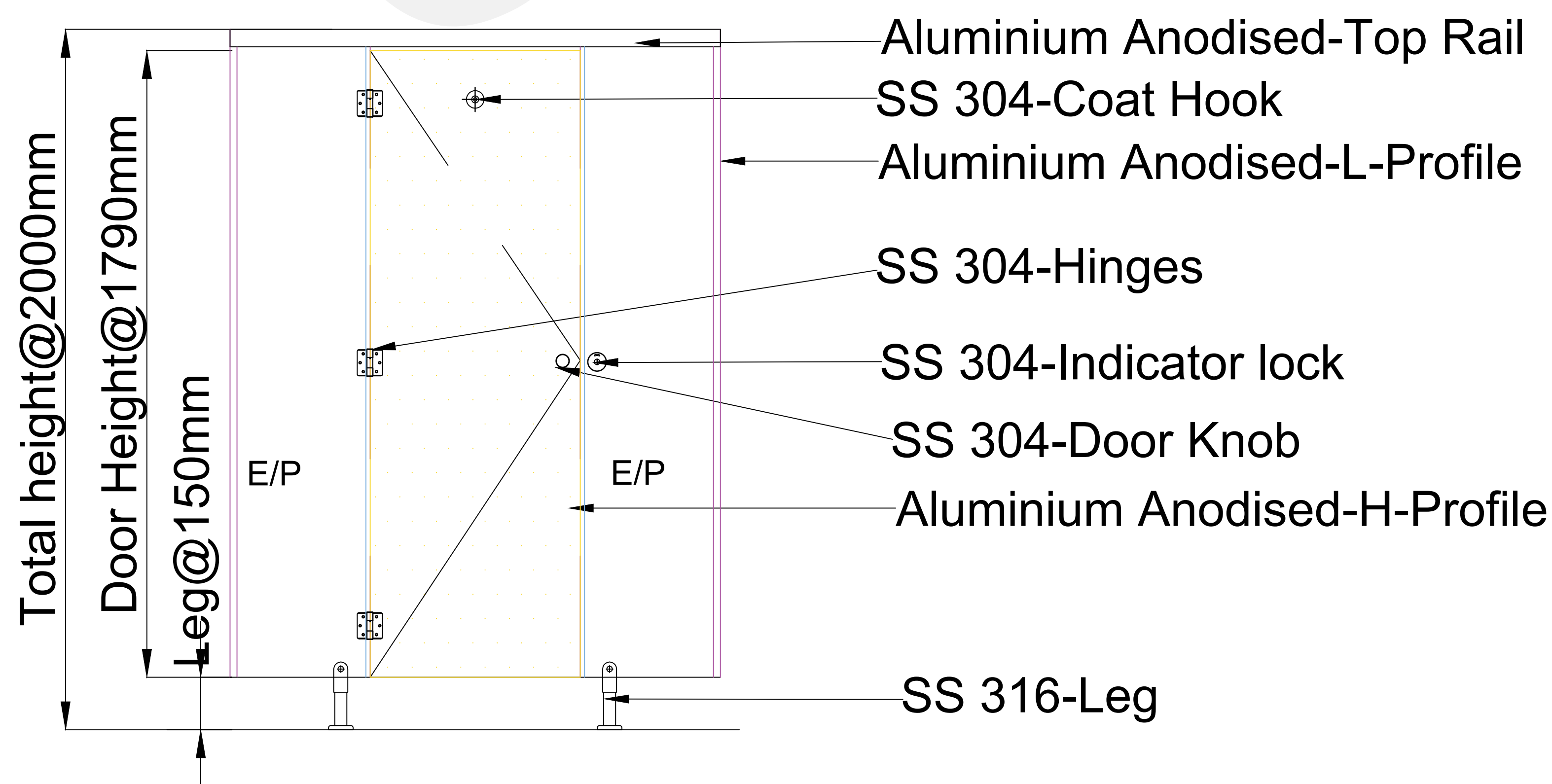
ELEVATION-AA
