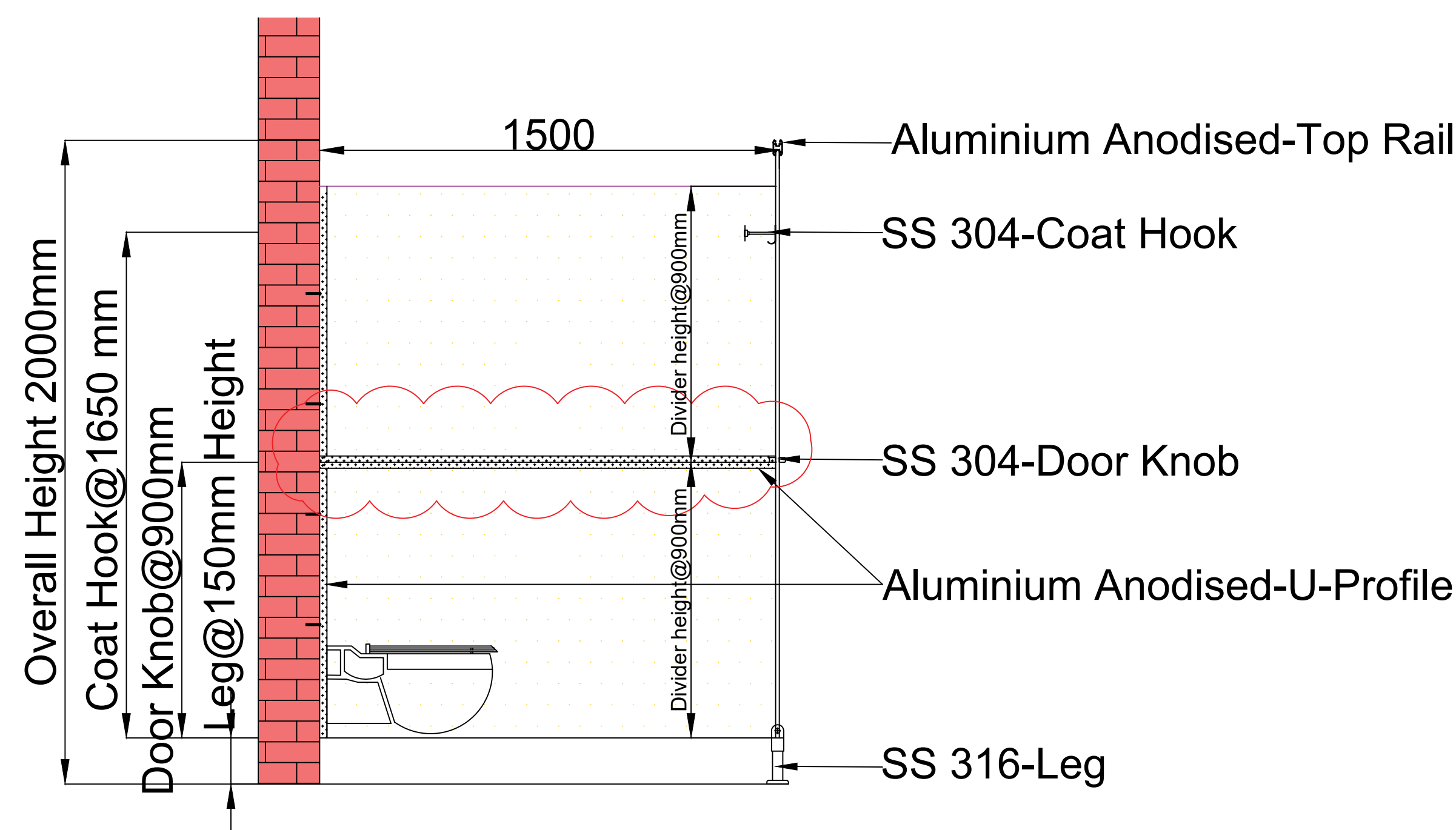
SECTION-BB
